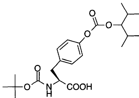
Fig.1. Boc-Tyr(Doc)-OH.
